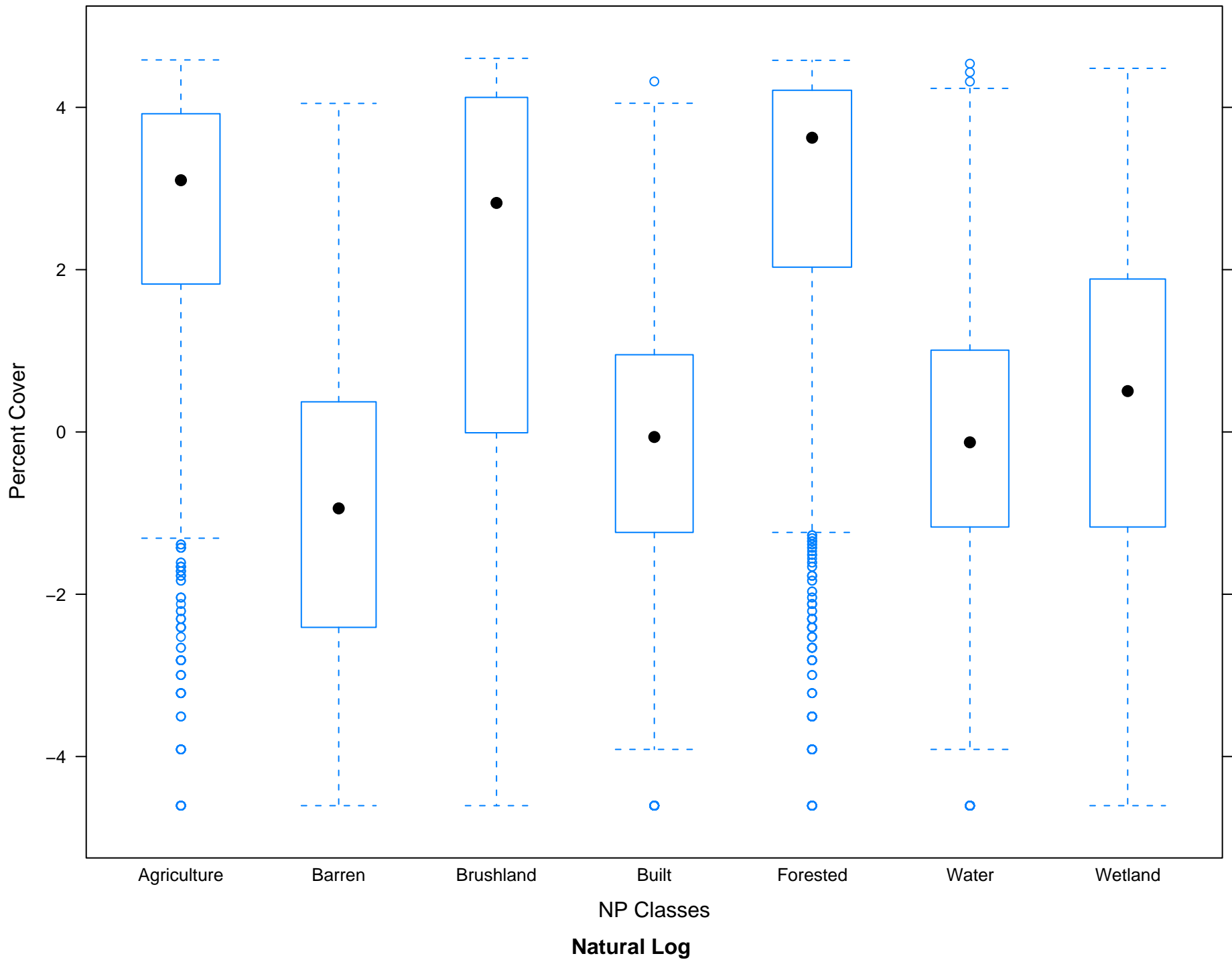
Boxplot of NLCD Class Percentages within 5 km Buffer
