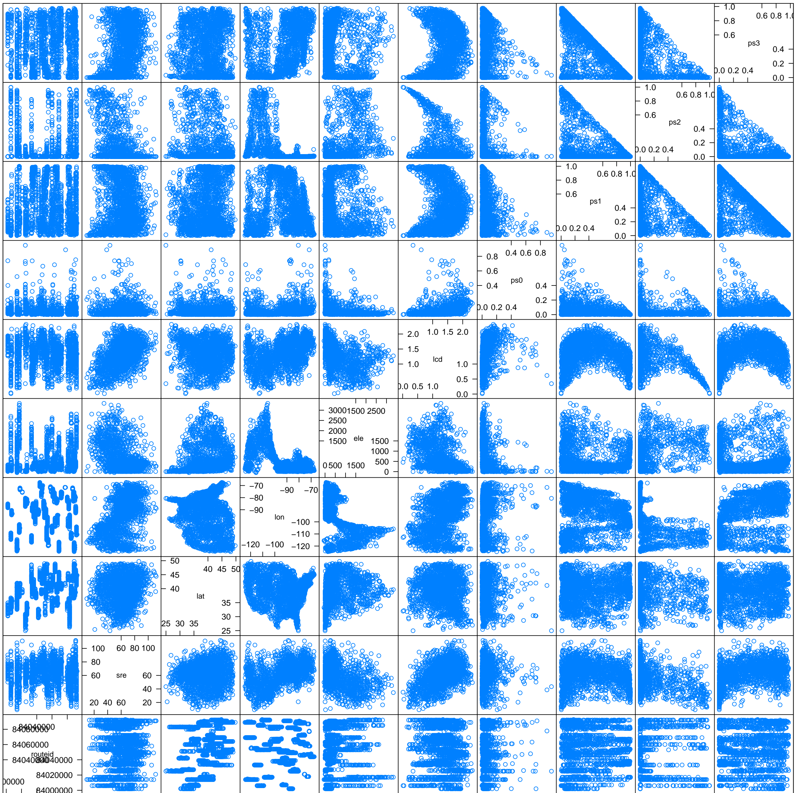
Scatter Plot Matrix
